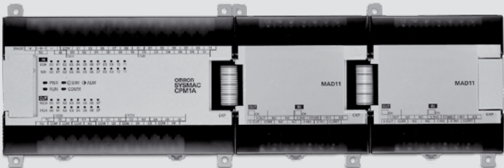
CPM2A CPU Unit with Two CPM1A-MAD11 Analogue I/O Units (2 Analogue Inputs and 1 Analogue Output)
